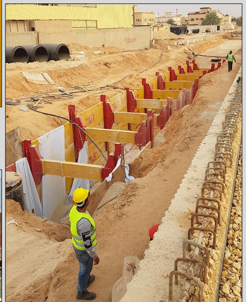
Double Slide Rail Shoring
