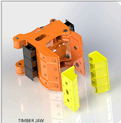
TIMBER JAW
